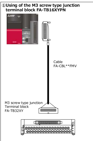
System architecture of alternative
